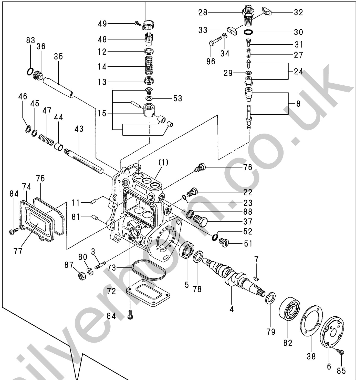
Fig. 11 FUEL INJECTION PUMP
