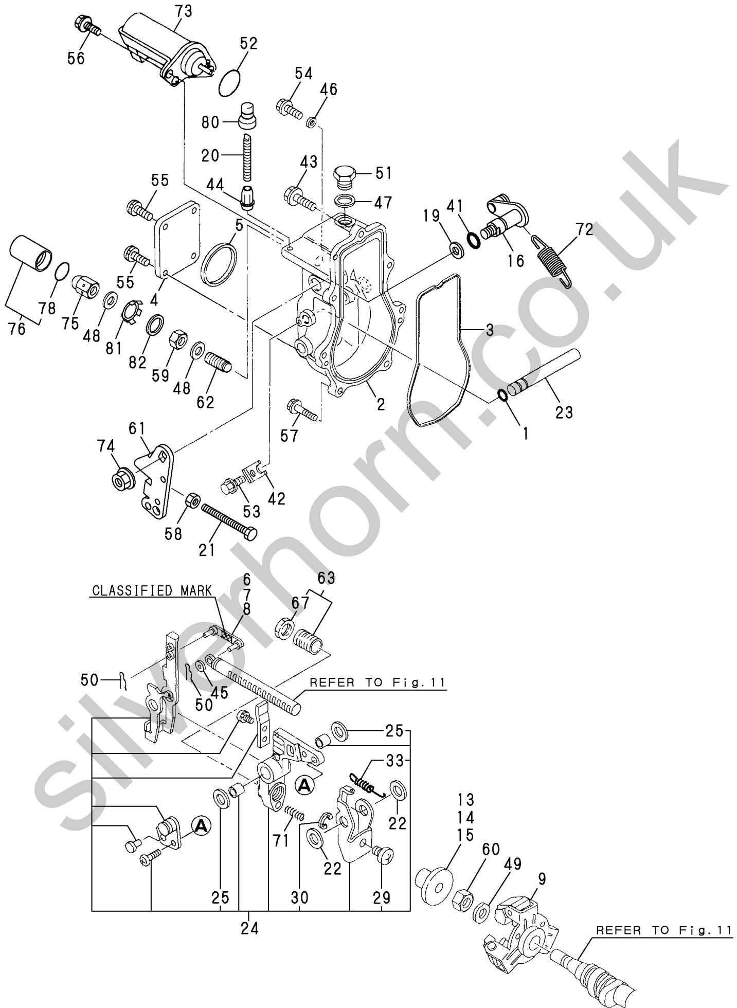
Fig. 12 GOVERNOR
