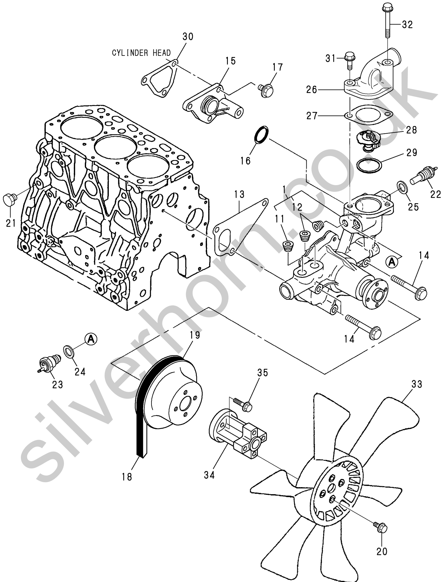
Fig. 10 COOLING WATER SYSTEM
