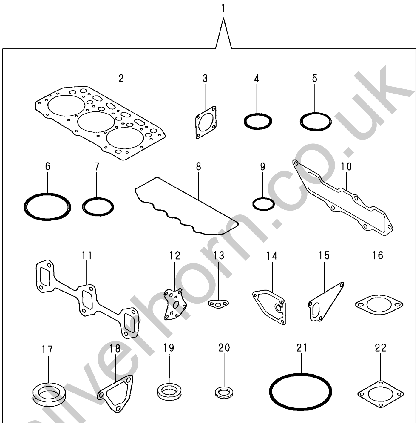
Fig. 17 GASKET SET & TOOLS
