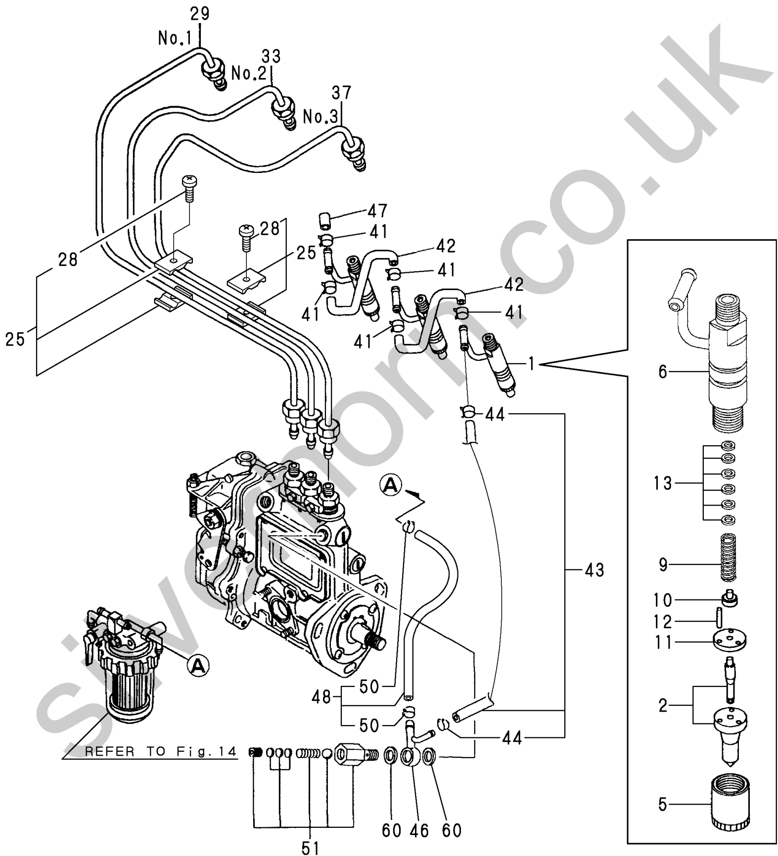
Fig. 13 FUEL INJECTION PIPE
