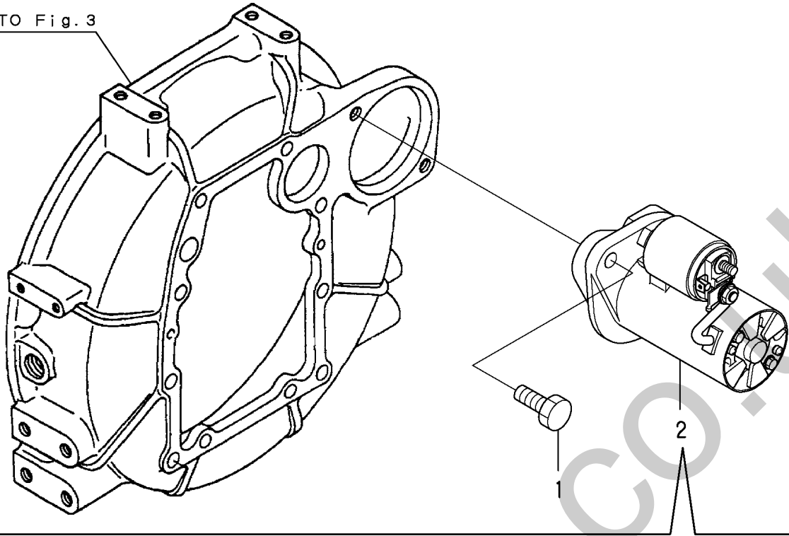
Fig. 15 STARTING MOTOR
